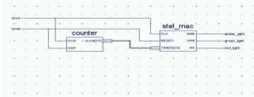
Figure 4.6.6 More Net Names
