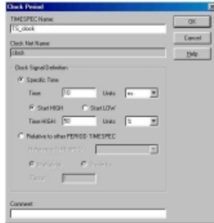
Figure 5.3.3 Clock Period Editor Window
