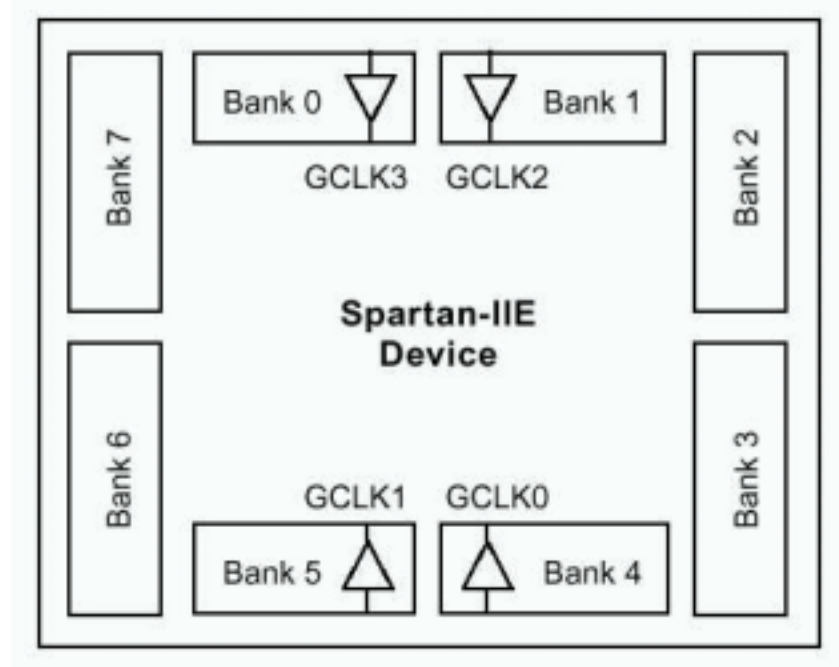
Figure 2.7 Spartan IIE Banking of I/O Standards
