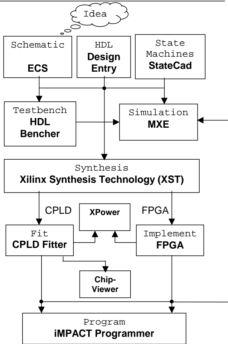
Figure 3.1 WebPACK Design Flow
