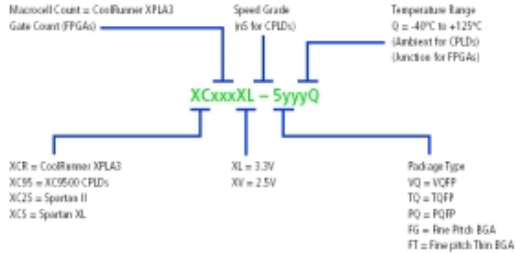
Figure 2.2.6 IQ Devices Ordering Information
