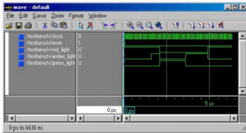
Figure 4.6.9 ModelSim Simulation Window
