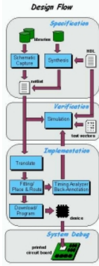
Figure 1.10 The PLD Design Flow
