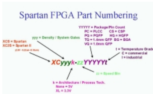
Figure 2.14 Spartan FPGA Part Numbering Guide
