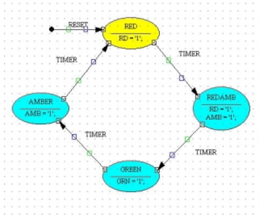
Figure 4.4.5 State Diagram
