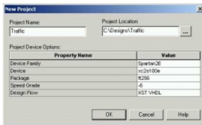
Figure 4.2.1 Project Properties Window CPLD designs
