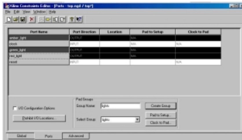
Figure 5.3.4 Constraints Editor – Create Group
