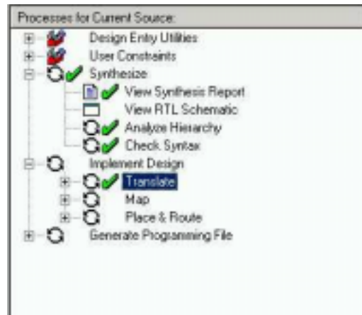
Figure 5.3.6 Design Process Window
