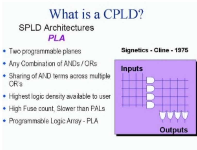
Figure 1.1 What is a CPLD?
