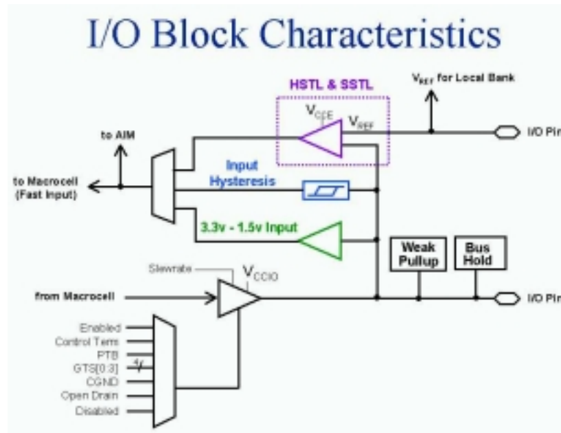
Figure 2.29 CoolRunner II I/O Block
