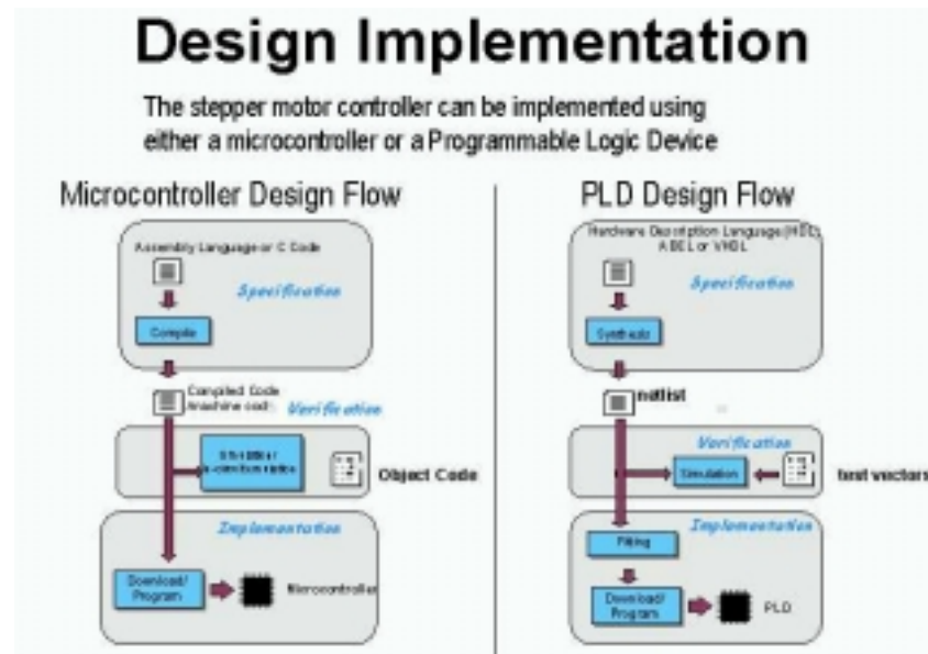
Figure 7.2.2 Design Flow Comparison
