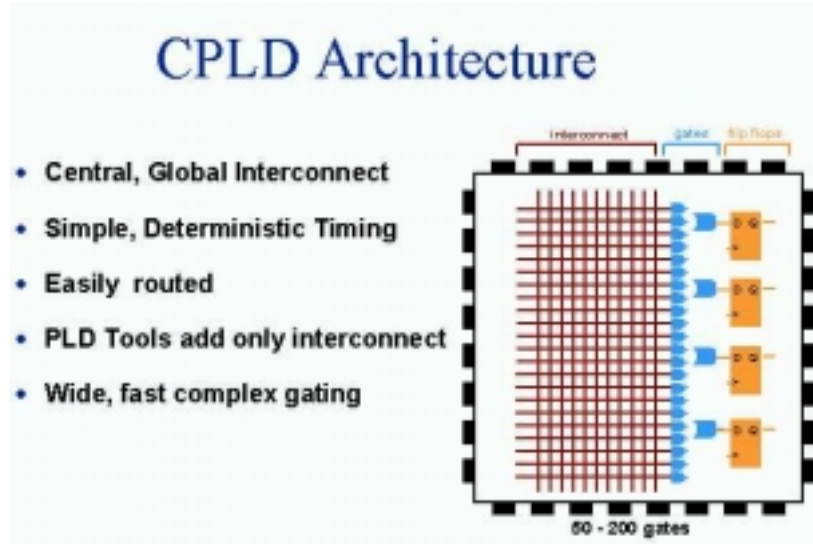
Figure 1.3 CPLD Architecture
