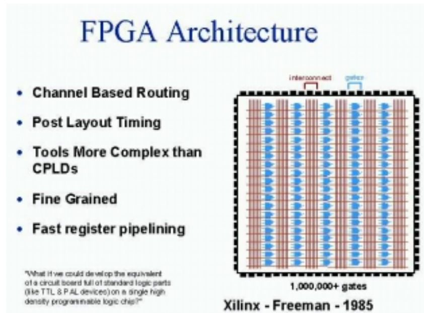
Figure 1.4 FPGA Architecture
