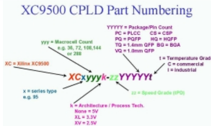
Figure 2.16 XC9500 CPLD Part Numbering System
