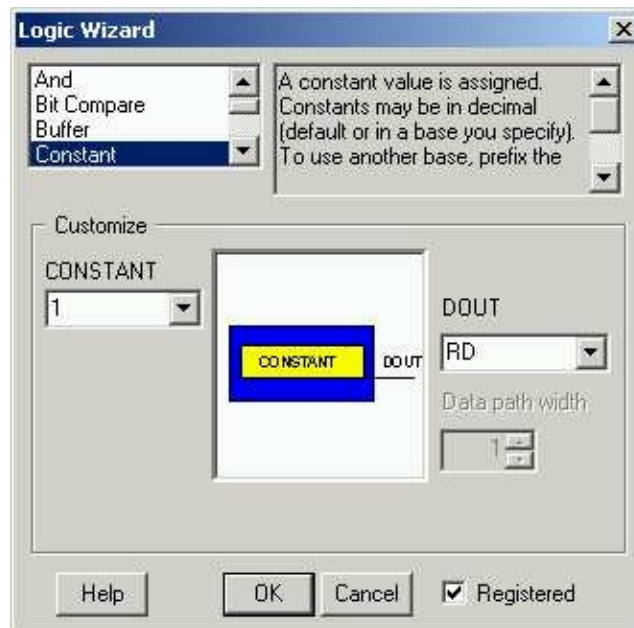
Figure 4.4.4 Logic Wizard Window
