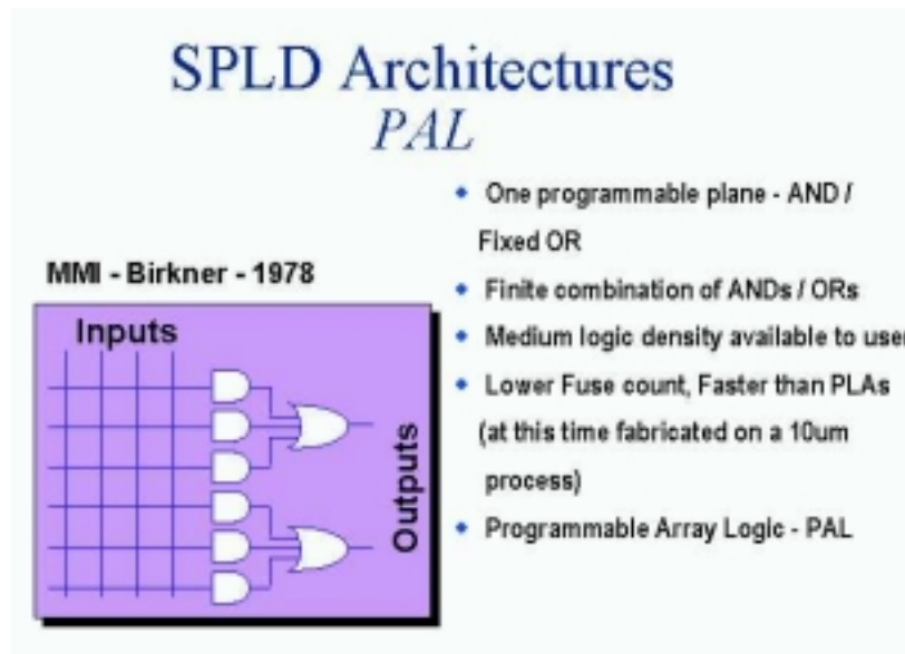
Figure 1.2 SPLD Architectures
