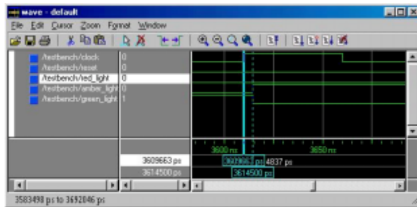
Figure 5.5.1 Simulation Window showing Timing
