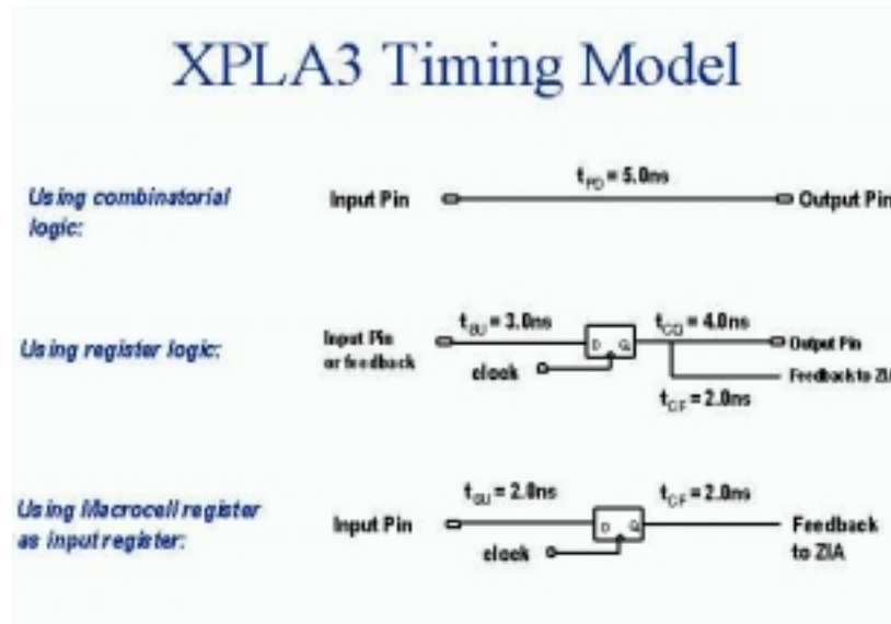
Figure 2.22 CoolRunner XPLA3 Simple Timing Model
