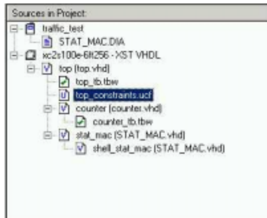
Figure 5.3.1 Constraints File as a source
