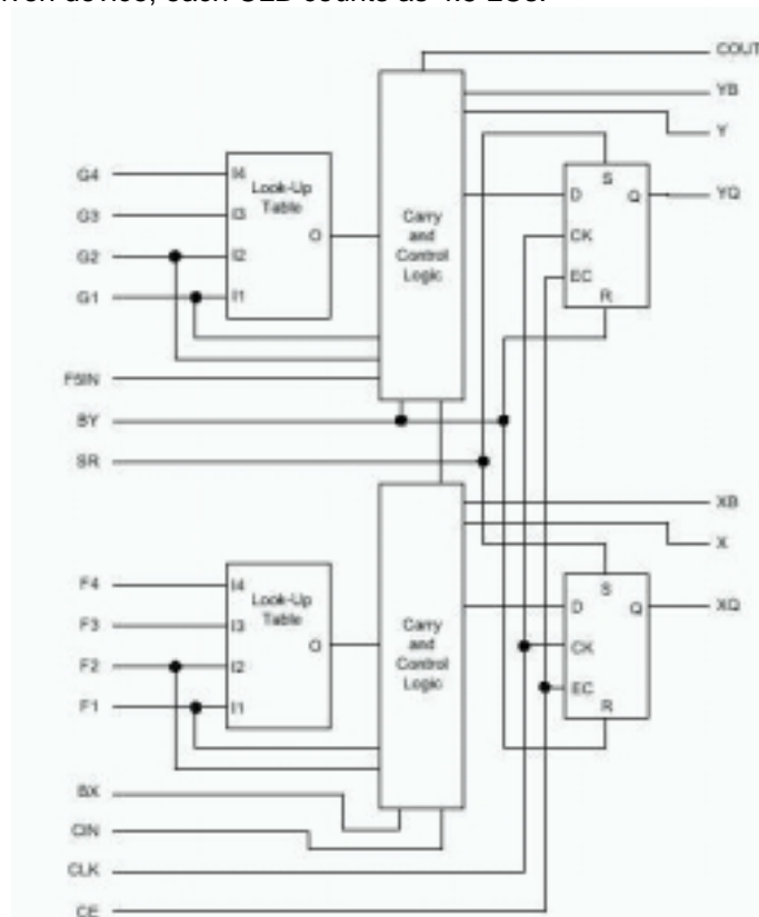
Figure 2.8 Spartan IIE Logic Cell
