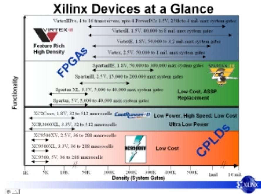
Figure 2.2 Xilinx Devices at a Glance
